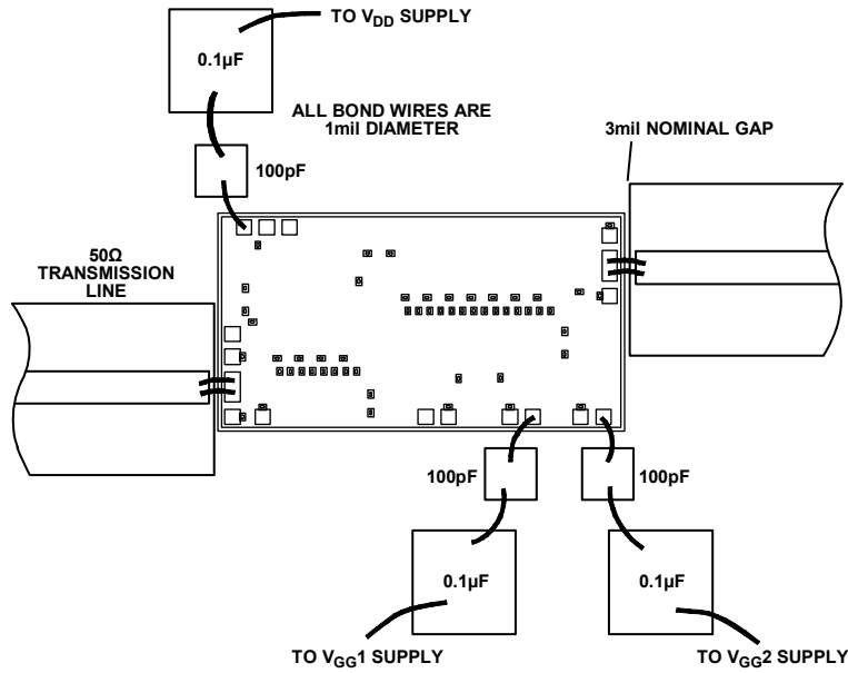
Figure 39. Assembly Diagram
