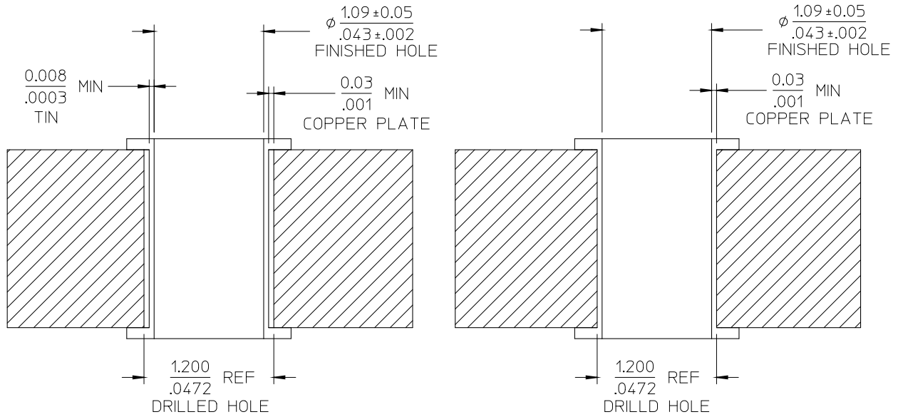
Sn/Cu PLATED HOLES
