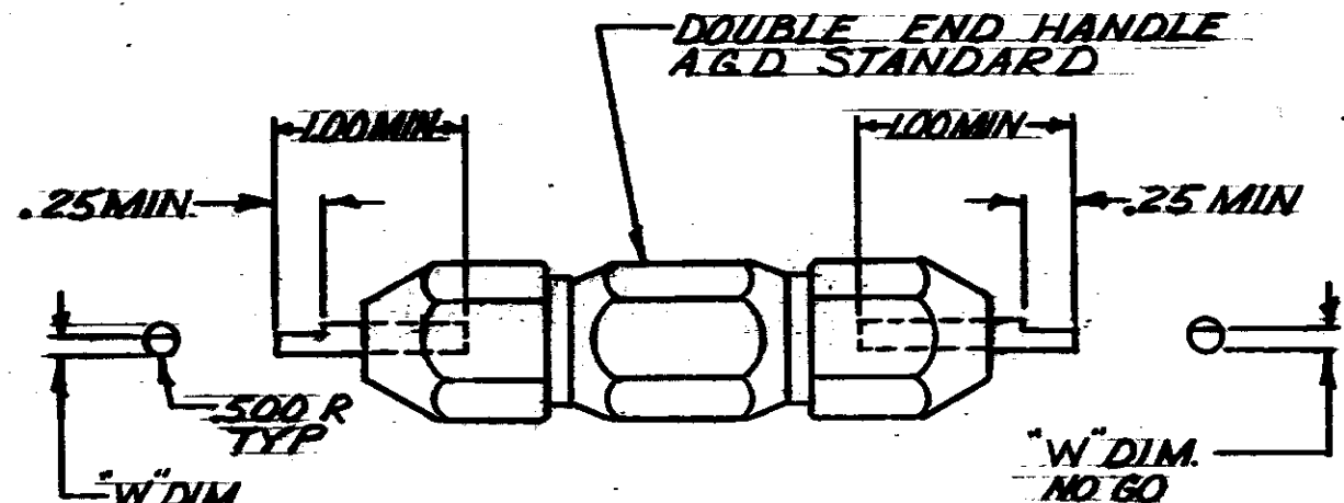
SUGGESTED PLUG GAGE FOR "W" CRIMP
