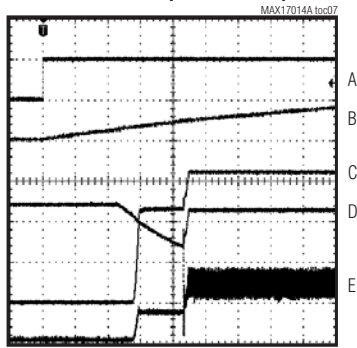
STEP-UP REGULATOR SOFT-START (HEAVY LOAD)
