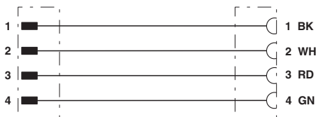
Contact assignment of 7/8\"-16UNF plugs/sockets
