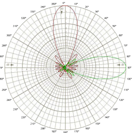
YA9W-13 at 960 MHz
