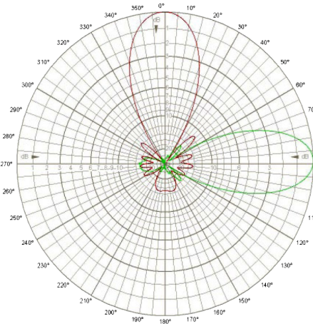
YA9W-11 at 960 MHz
