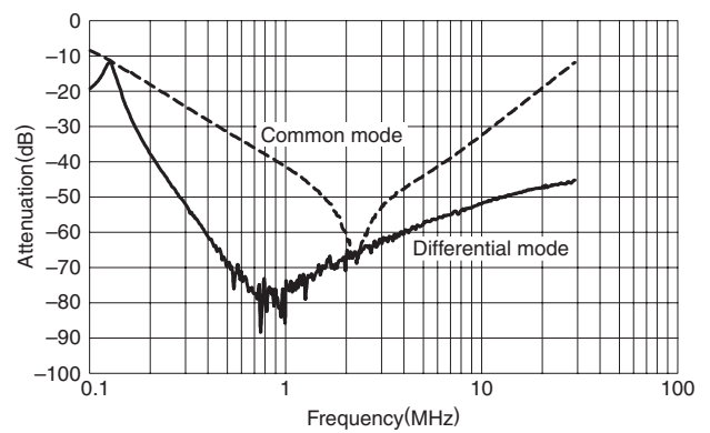
RTAN-5030
