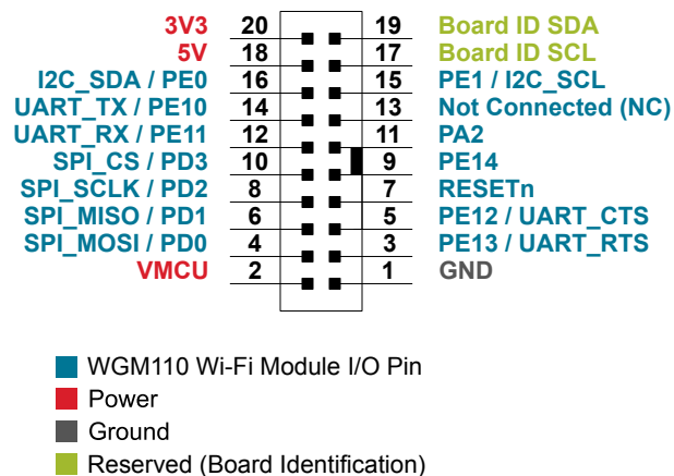
Figure 4.2. Expansion Header
