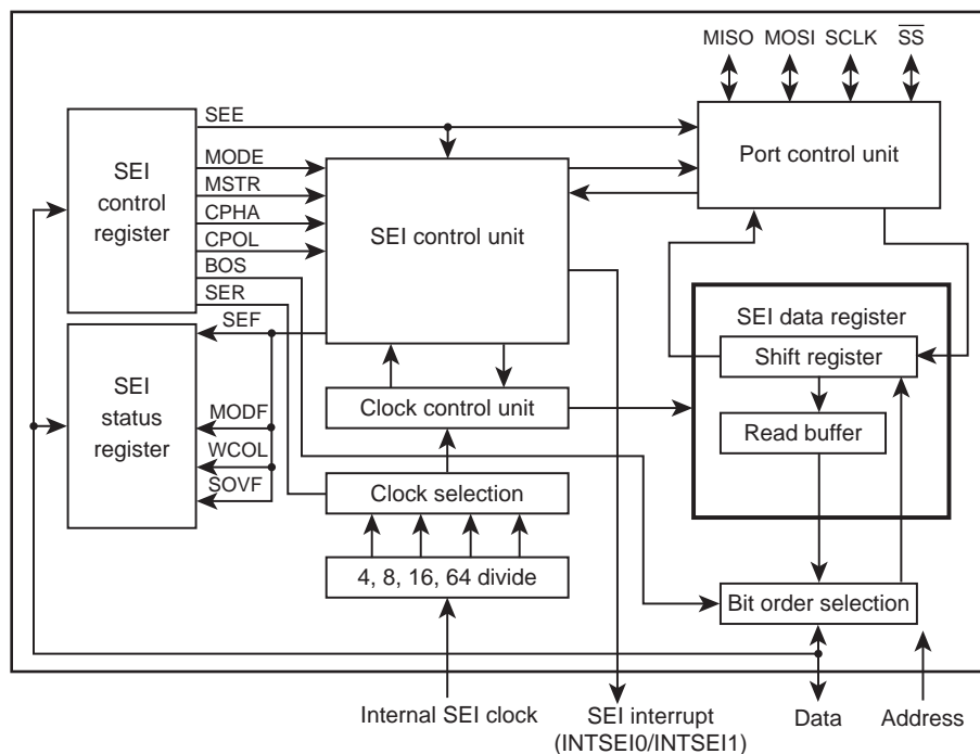
Figure 14-1 SEI (Serial Extended Interface)
