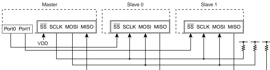
Figure 14-5 Example of SEI System Configuration (1 Master, 2 Slaves)
