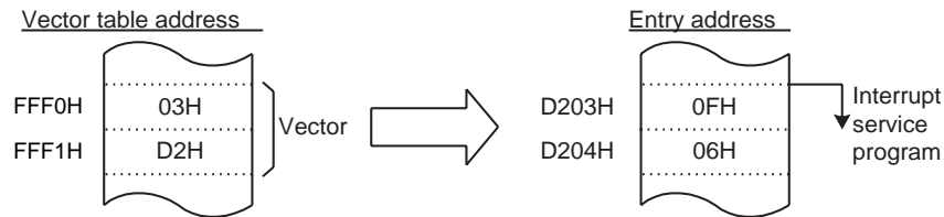
Figure 3-2 Vector Table Address and Entry Address
